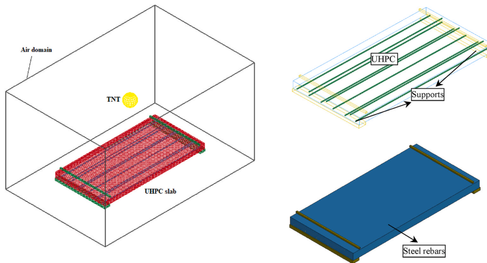
Fig. 10. UHPC Slab configuration and reinforcement.
